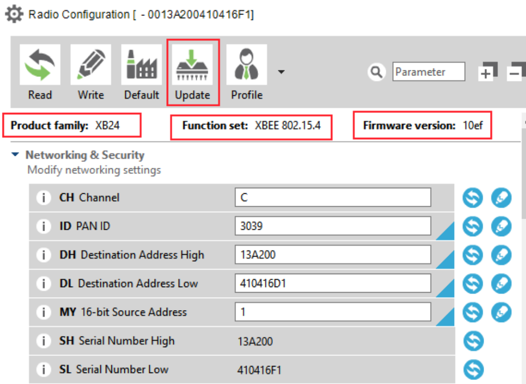
Figure 20: Firmware for XBee
