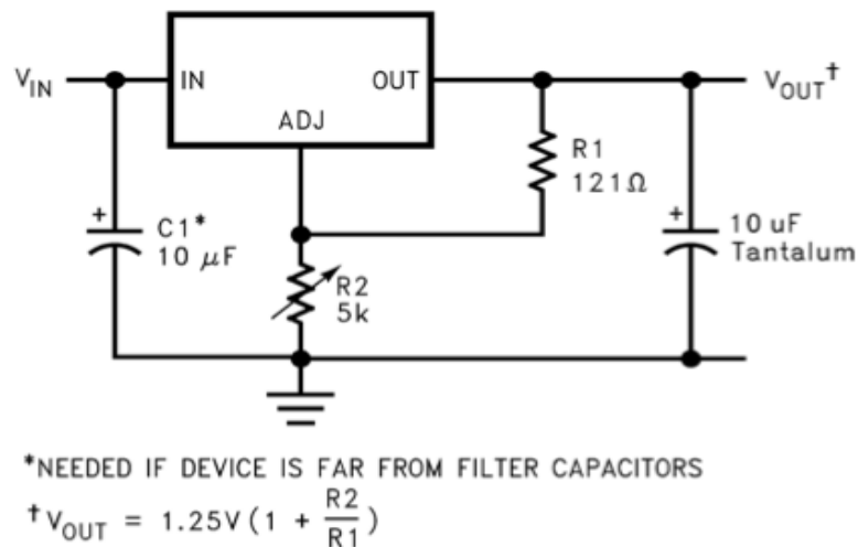
Figure 11: LM1084 Schematic with Formula. Permission Granted Courtesy of Texas Instruments
