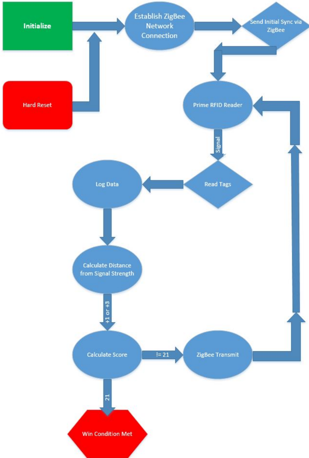
Figure 21: Main Gameboard Software Flowchart
