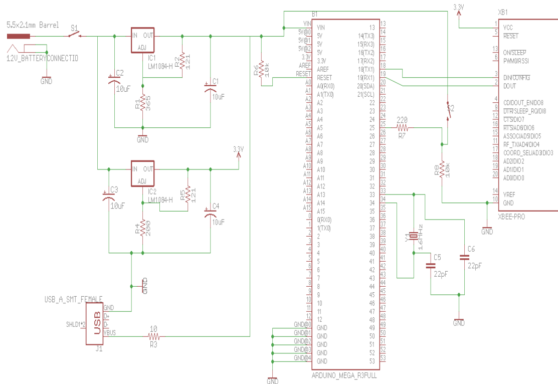
Figure 20: Module MCU with ZigBee Schematic
