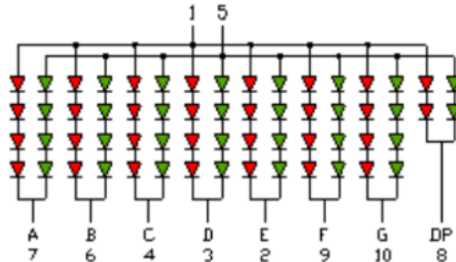
Figure 24: Pin setup for 7-segment displays
