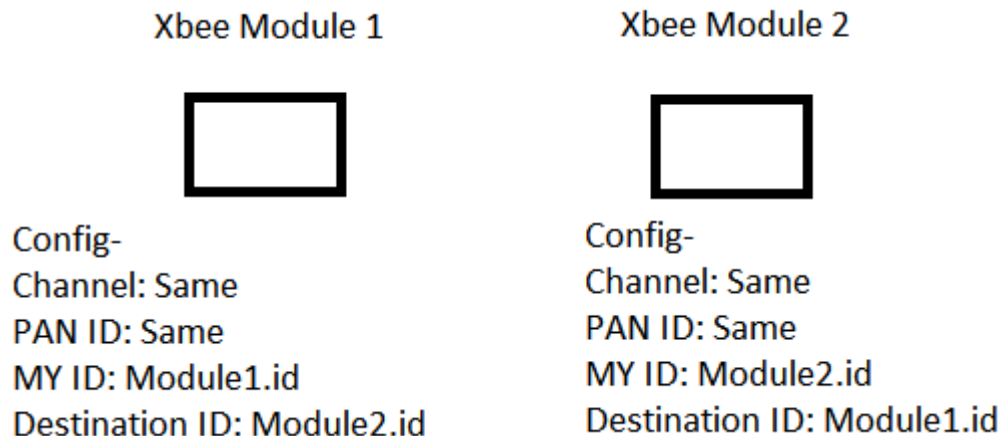
Figure 12: Xbee Configuration
