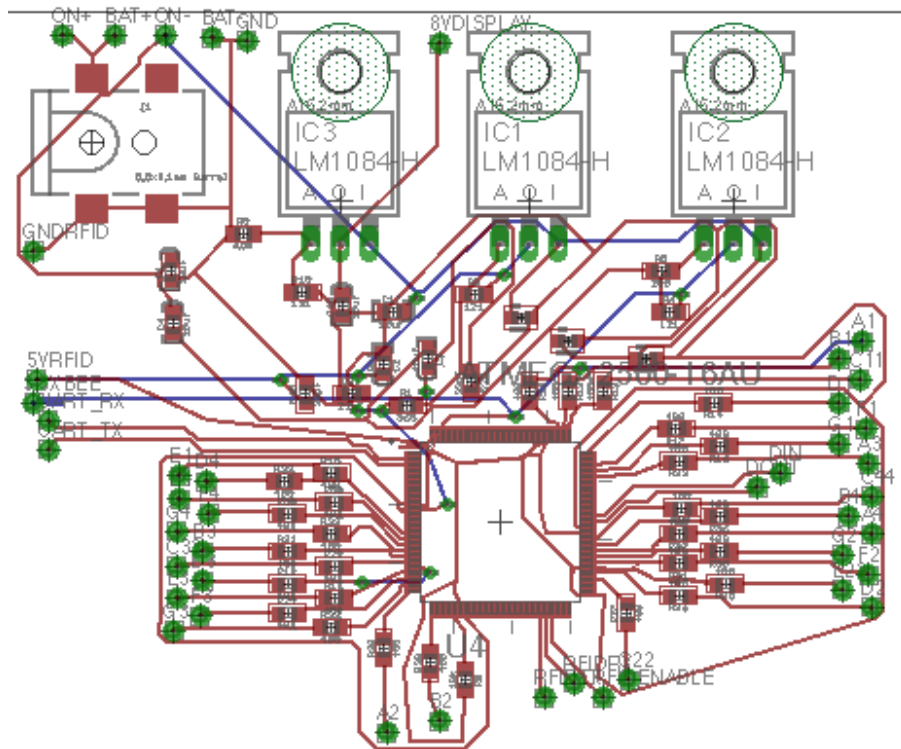
Figure 27: Game board Prototype PCB
