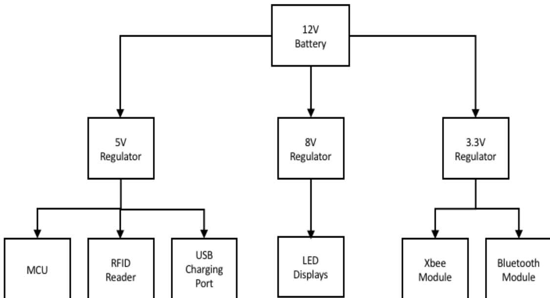
Figure 10: Power system of the Smart Cornhole
